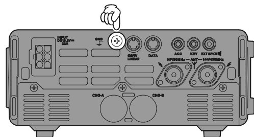
GND Terminal
